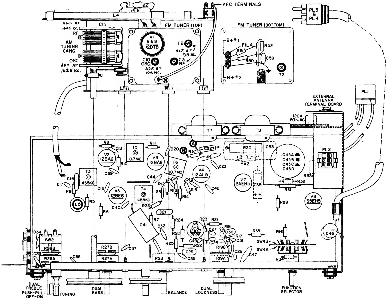
Top View of V-2515-11 Chassis
